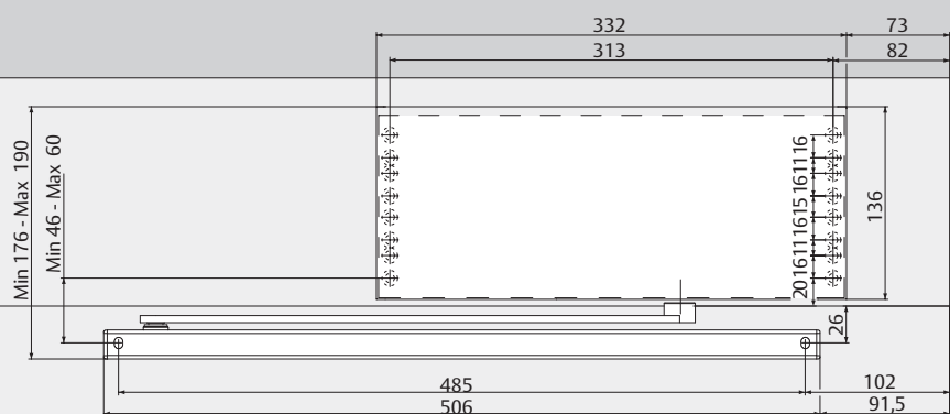
Non-hinge side installation on frame Max. opening angle \sim 125^\circ
