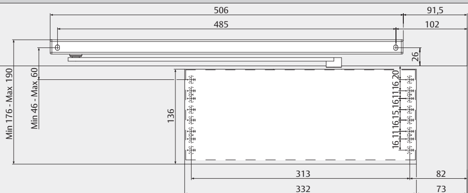
Hinge side installation on door Max. opening angle \sim 180^\circ
