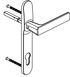
DIN LH02751 Outside single handle (with inside panic bar)
