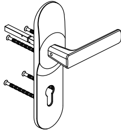
DIN LH0241 Outside single handle (with inside panic bar)
